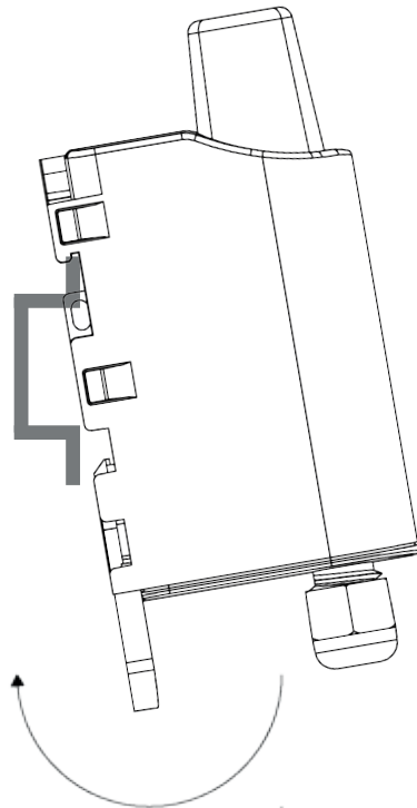
Rail-DIN locking
